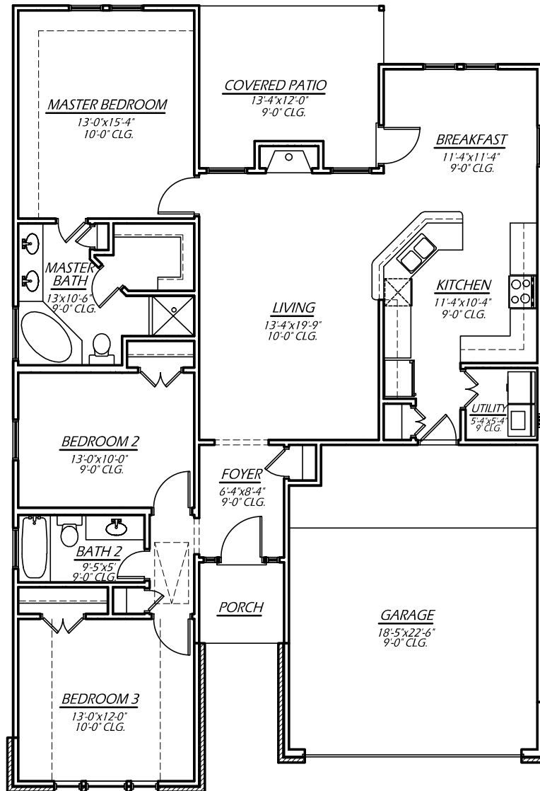
Floor Plan A
